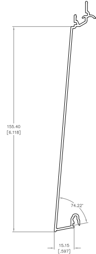
P96L - LAP ALUMINUM TRIM SYSTEM PROFILE
