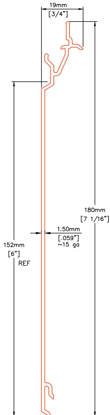
P46V V-NOTCH 6" PLANK
