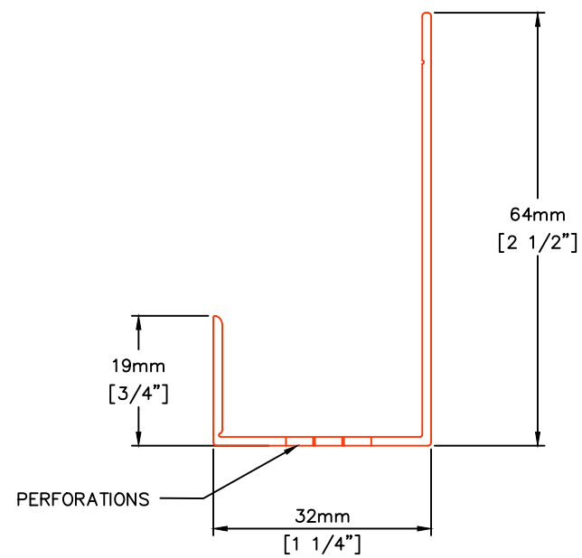
P41 PERFORATED STARTER J
