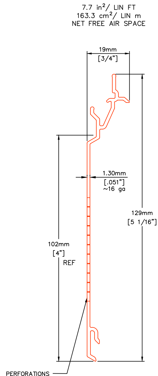
P47V V-NOTCH SOFFIT PLANK
