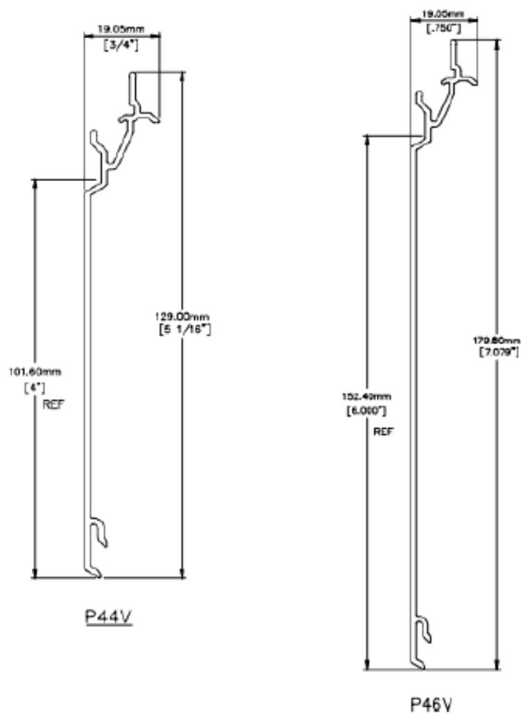
FIGURE 1 – PLANK DIMENSIONS
