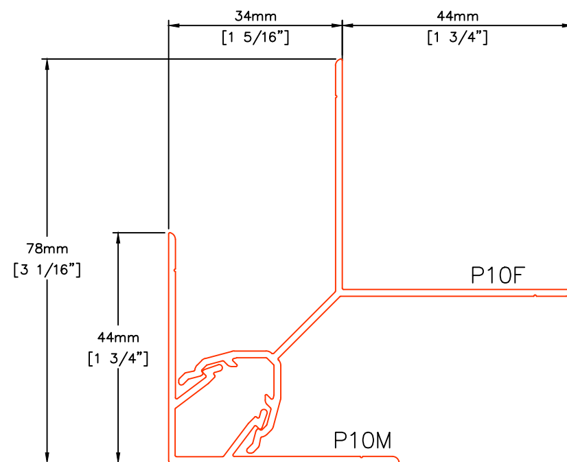
P10 INSIDE/OUTSIDE CORNER
