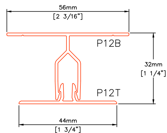
P12 2-PIECE VERTICAL
