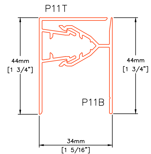
P11 2-PIECE J
