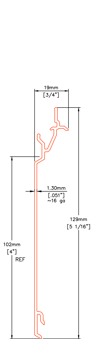
P44V V-NOTCH 4" PLANK
